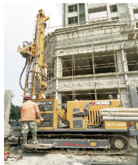
XSL5/260水井钻机湖北地热井施工 XSL5/260 Water Well Drilling Rig in Geothermal Well Construction in Hubei
